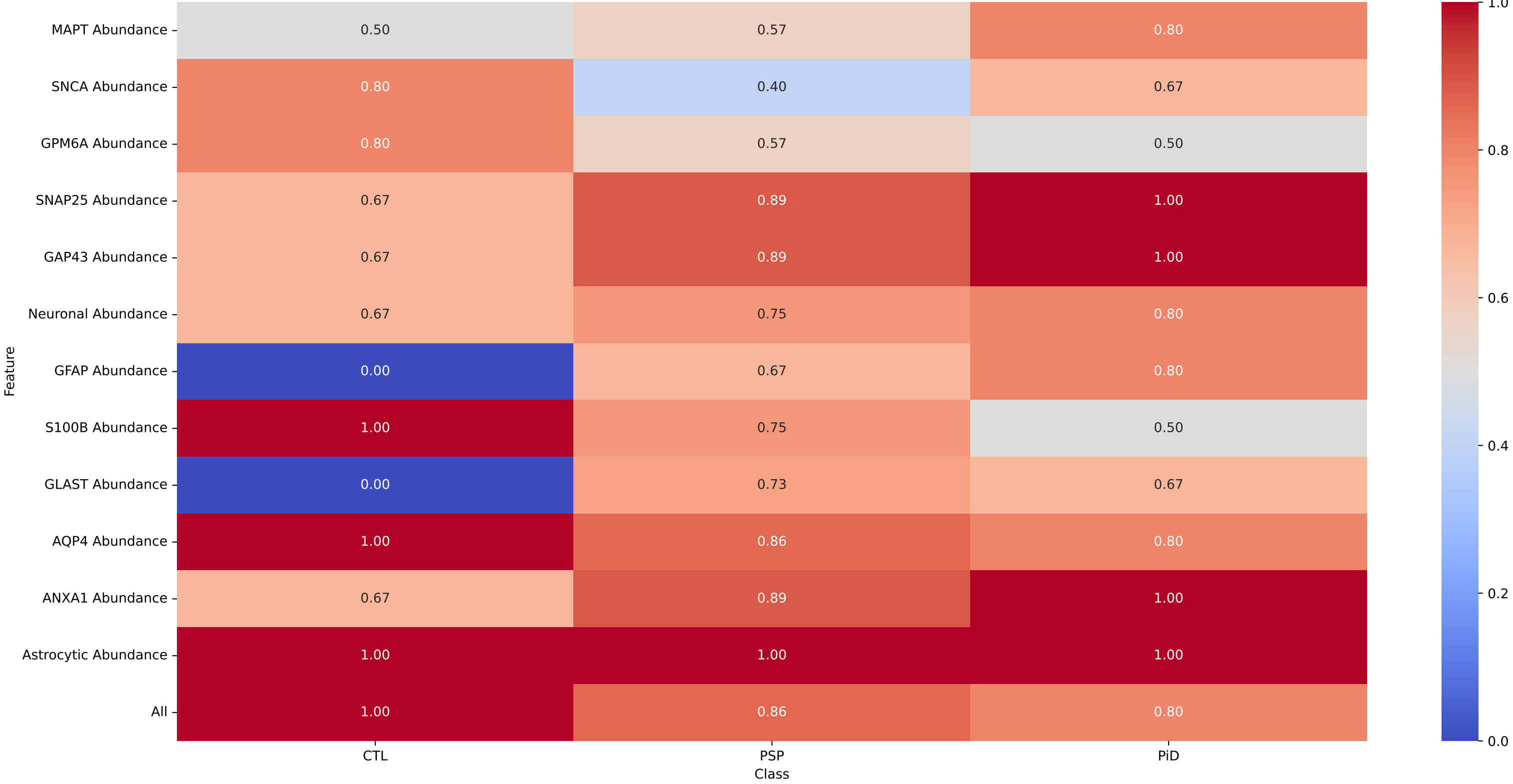
Predictive Classification
